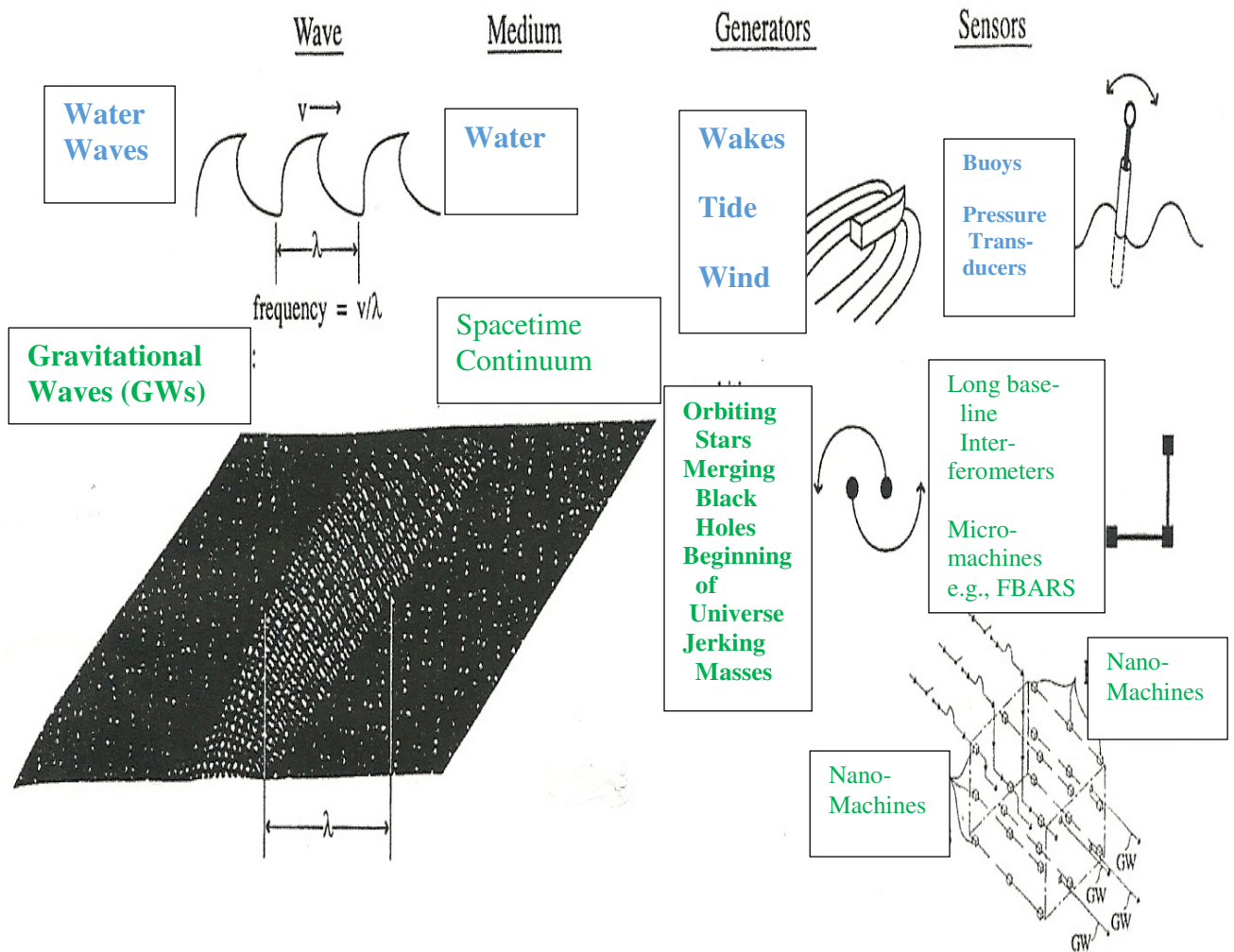
Figure 5. Gravitational waves.
