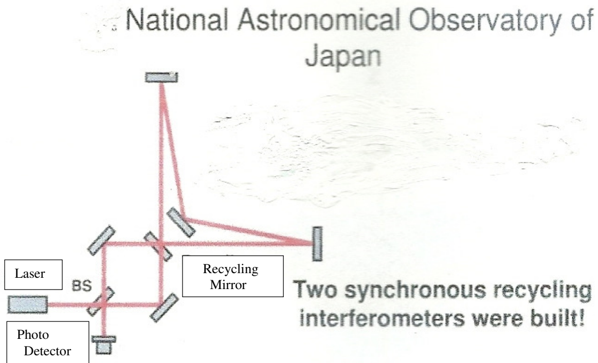
Figure 8. National Astronomical Observatory of Japan 100 MHz HFGW Detector (Nishizawa, et al. , [70]).
