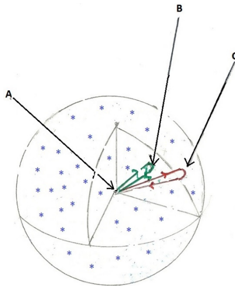
Figure 4. The boundary sphere of radius 5000 light years containing stars in the neighborhood of our Sun whose advanced civilizations could intercommunicate.
