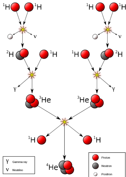
Figure 6. Standard diagram of proton-proton chain reaction.
