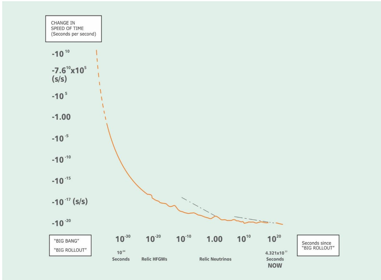
Figure 2. Notional graph from Fig. 3 of [11] of the change-of-speed-of-time variation with today's time dimension. The Figure is only a schematic and not intended for detailed analyses. Notice different slopes (tangents) and irregularities and the current time rate of about 10^{-17} seconds per second between 10^{-15} and 10^{-20} seconds per second shown by the expanded graduation scale on the ordinate near the "BIG BANG" or "BIG ROLLOUT".
