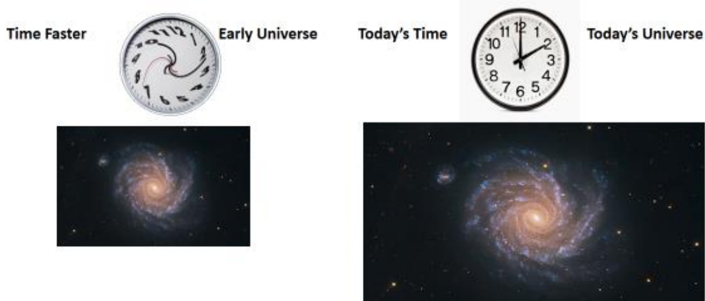
Figure. 3, Rotational rate of galaxies.
